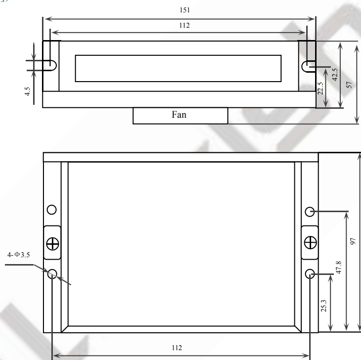
Figure 1: Mechanical specifications
