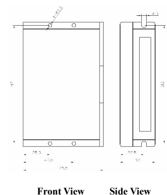
Figure 1: Mechanical specifications
