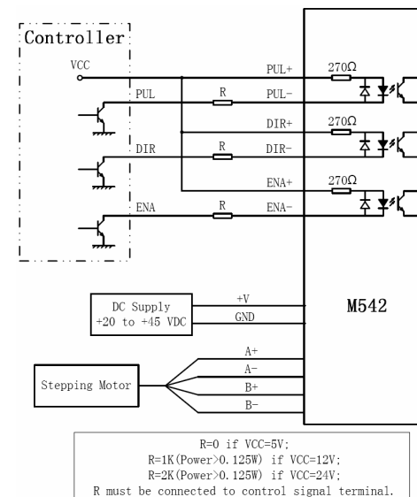
Figure 3: Typical connection
